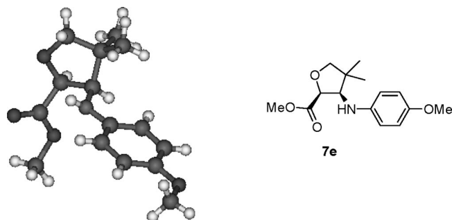
Figure 2. X-ray analysis of methyl cis -3-(4-methoxyphenylamino)-4,4-dimethyltetrahydrofuran-2-carboxylate ( 7e ).
