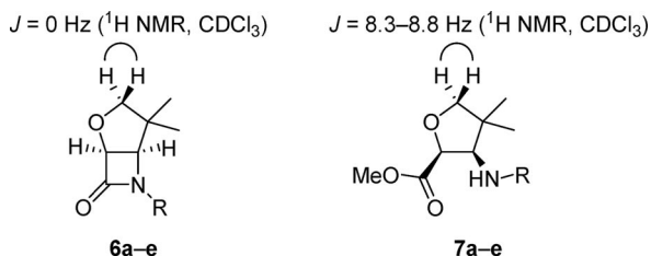
Figure 1. Geminal coupling constants in oxolanes 6 and 7 .
